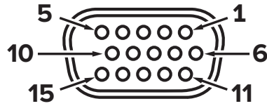
Female Connector: Device
