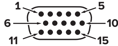
Male Connector: Cable
